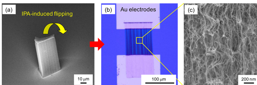
Figure 4. (a) Patterned nanotube forests on SiO 2 substrate. (b) Optical image of a forest after flipping and electrode definition. (c) SEM image showing the nanotubes after evaporation; the nanotubes appear to exhibit very low compaction.
