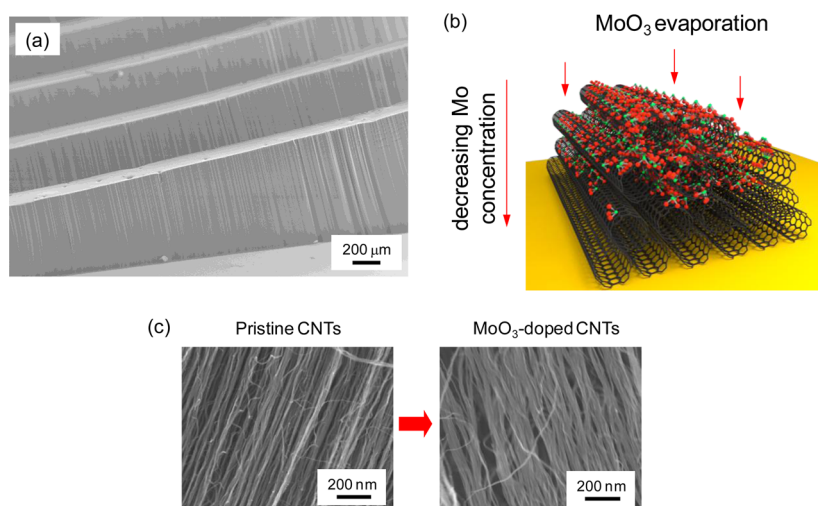
Figure 3. (a) SEM image of gradient-height forests. (b) Schematic for MoO 3 evaporation in one direction. (c) SEM image of a nanotube bundle prior to and after doping.
