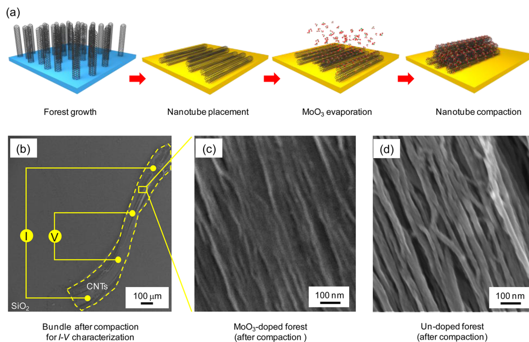
Figure 1. (a) Schematic of techniques employed for nanotube forest doping. (b) Optical image of nanotubes peeled off from a forest and compacted for electrical characterization. (c, d) Compacted forests after MoO 3 doping and pristine state, respectively.
