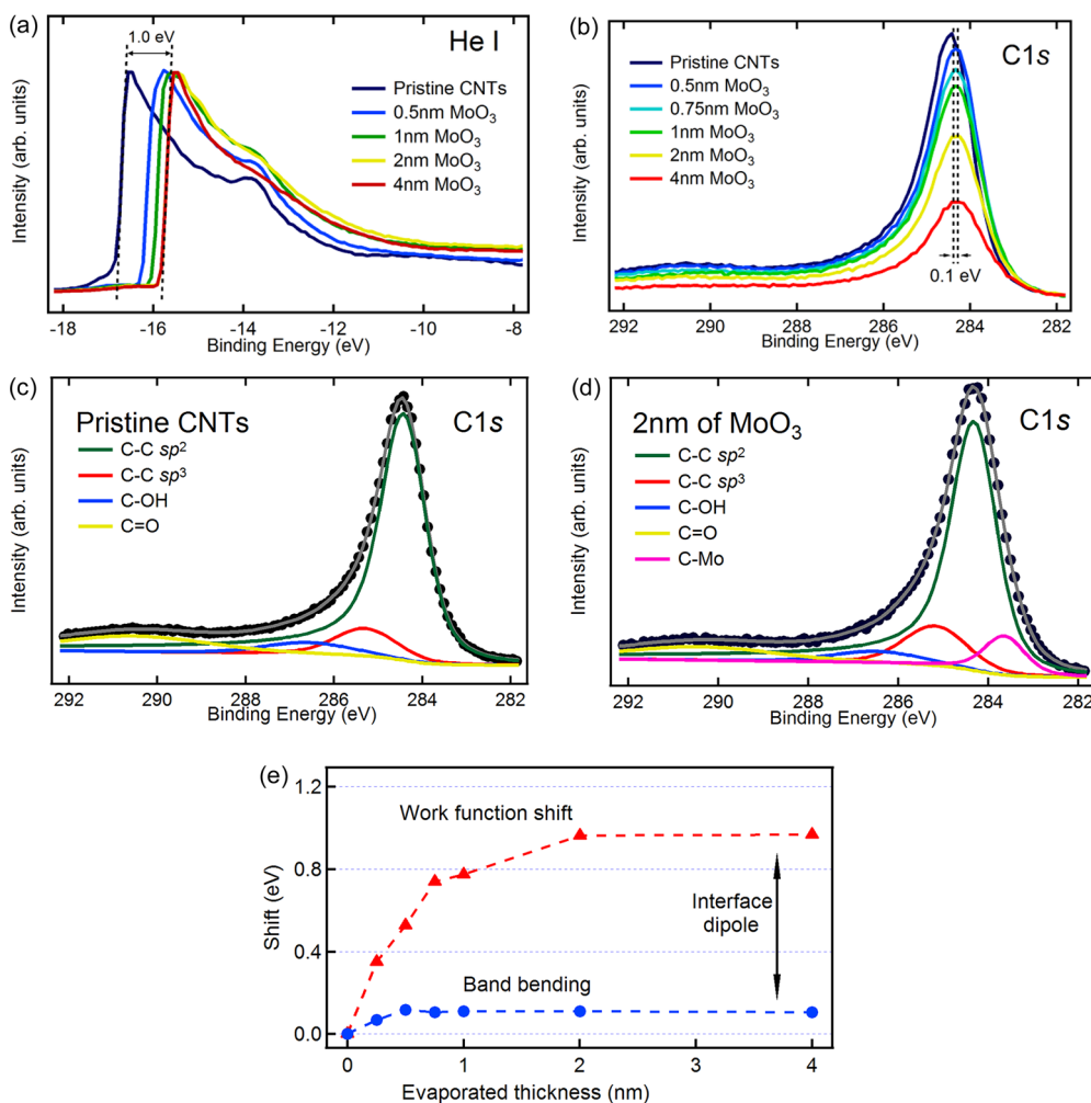
Figure 5. Variation of the secondary cutoff in UPS spectra, related to the shift of the forest work function. (b) XPS spectra of the C 1s aligned to the Fermi energy. (c, d) C 1s core level spectra before and after the evaporation of 2 nm MoO 3 . (e) Comparison of work function shift and band bending for different thicknesses of evaporated MoO 3 .
