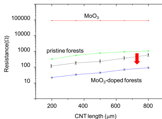
Figure 2. Resistance for doped and pristine nanotubes as a function of different forest length. The dashed line shows resistance values obtained when probing both doped and undoped tubes.
